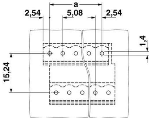
Drilling diagram
